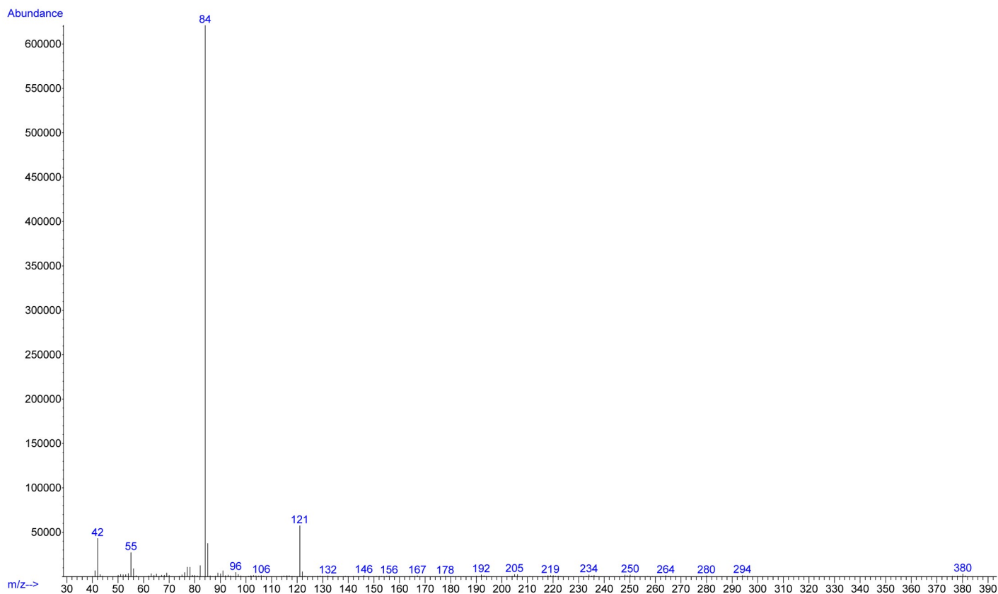
Mass Spectrum (EI 70 eV)
